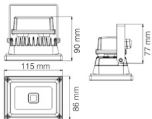
[FZL-FL12-00-12]
