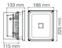
[FZL-FL35-00-35]
