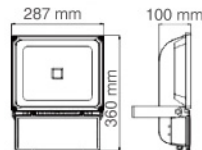
[FZL-FL110-00-110]
