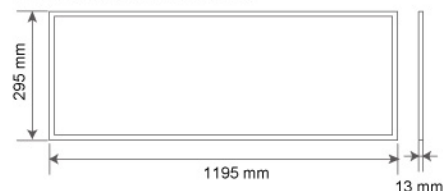
FZL-PL120-00-52 Series
